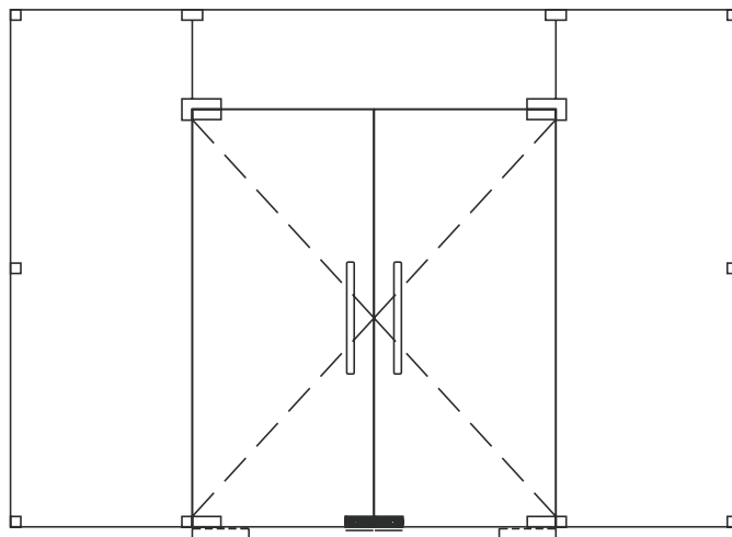
Corner Lock with EPC and strike plate
