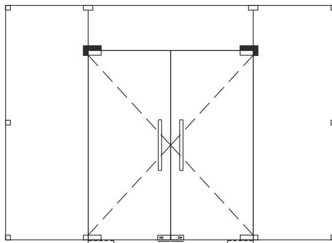
Patch fitting for overpanel and sidelight
